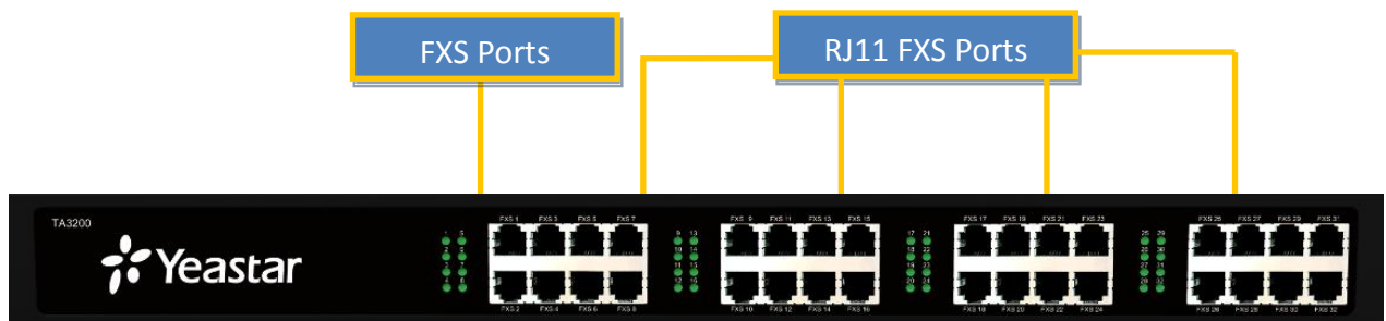
Figure 2-3 TA3200 Front Panel
