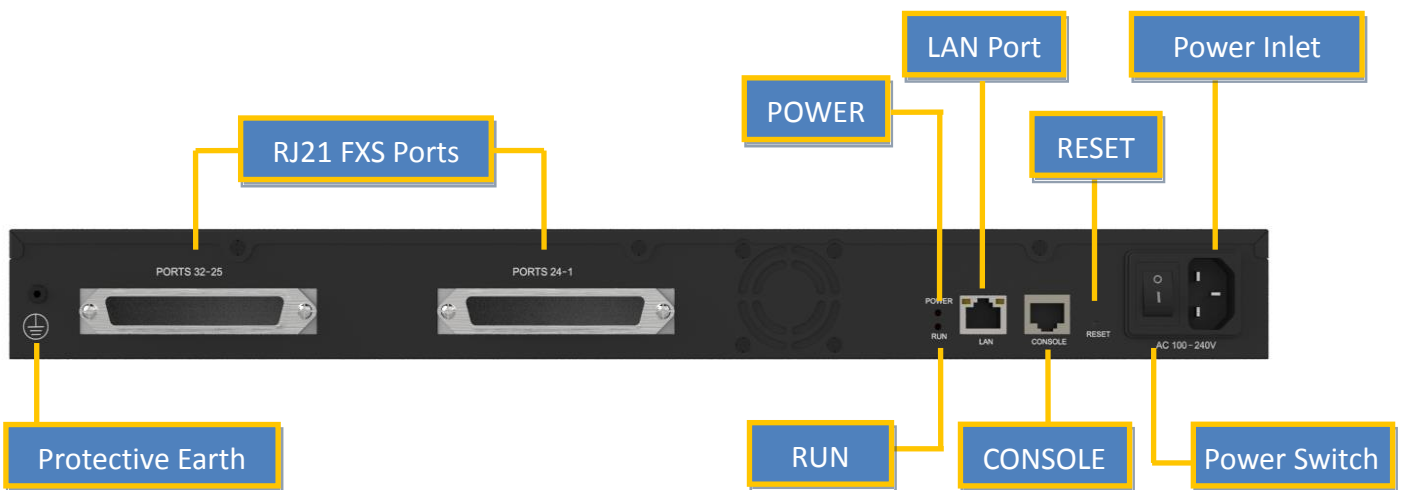
Figure 2-5 TA3200 Rear Panel
