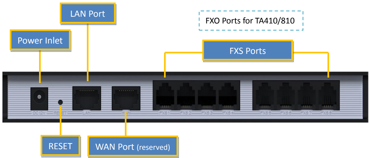
Figure 2-4 TA800 Rear Panel
