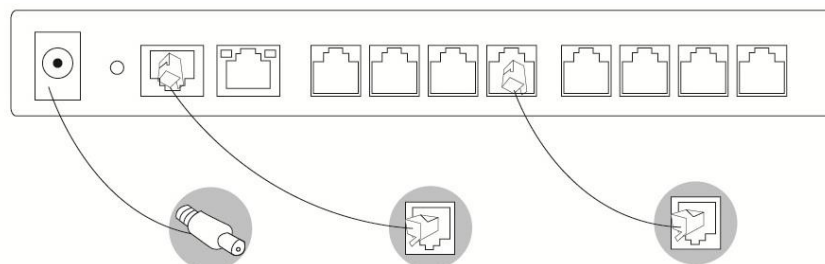
Figure 3-2 TA810 Connection Diagram
